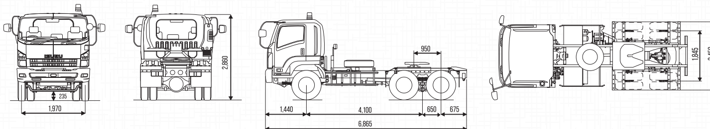
CONTAINER TRANSPORTER
